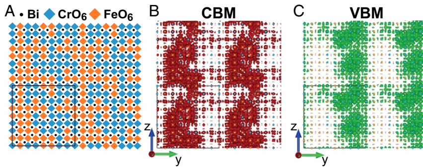
Fig. 3. Distinct e - h separation in disordered BFCO on a large scale. (A) Schematic of the tested 8 \times 8 \times 2 supercell. (B and C) Partial charge densities of the (B) CBM (in the red cloud) and (C) VBM (in the green cloud) states. CBM and VBM states are spatially separated onto the Fe-rich vs. Cr-rich domains, respectively.
