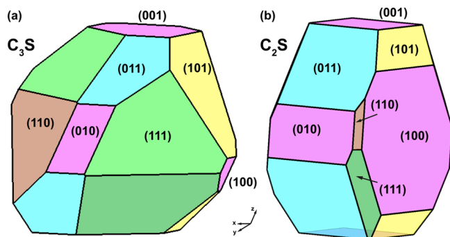
Figure 5. Wulff shapes of (a) C_3S and (b) C_2S based on the calculated surface energies for all low-index orientations (Table 1).
